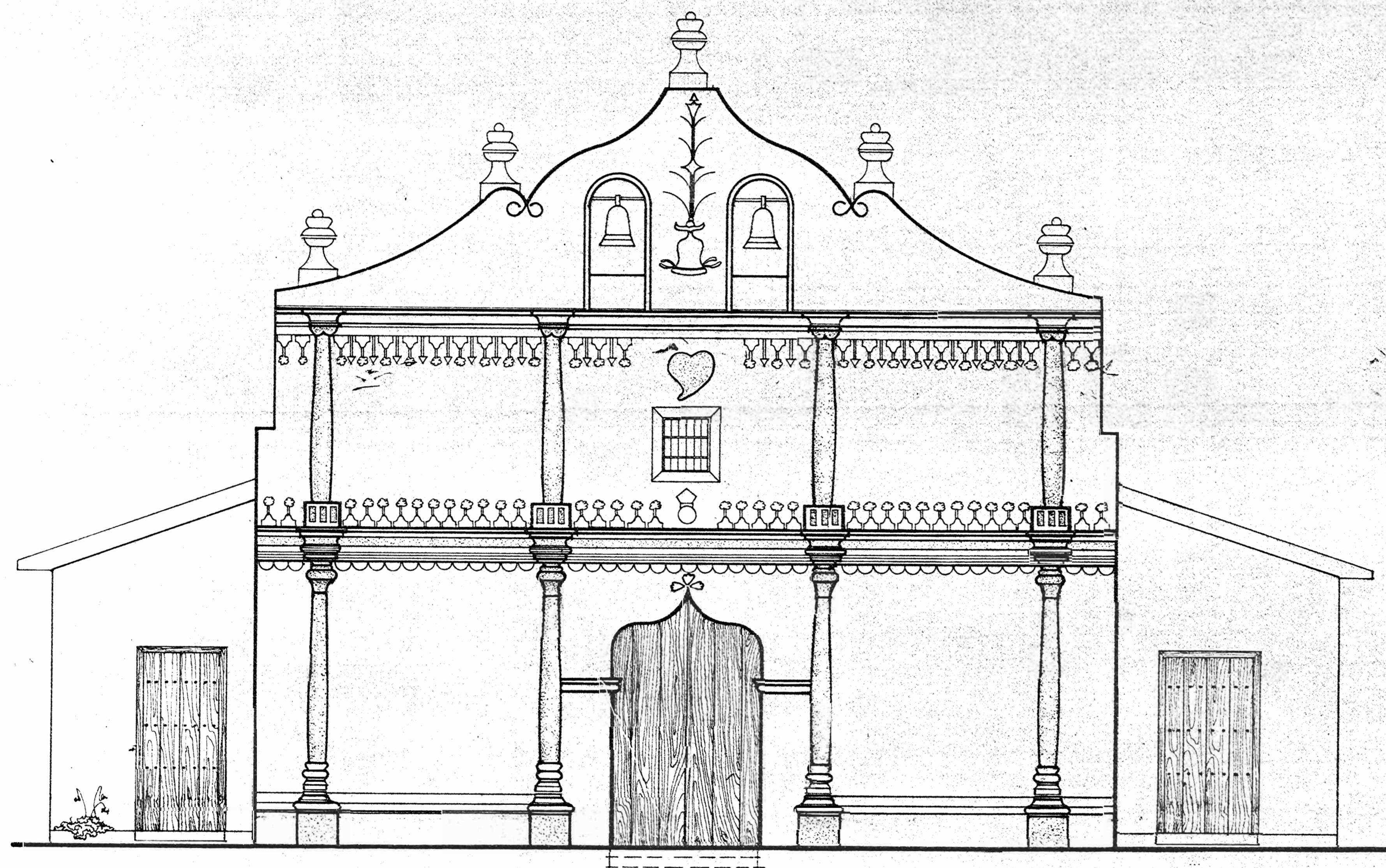
ELEVACION PRINCIPAL "RESTAURADA" Escala 1:50
