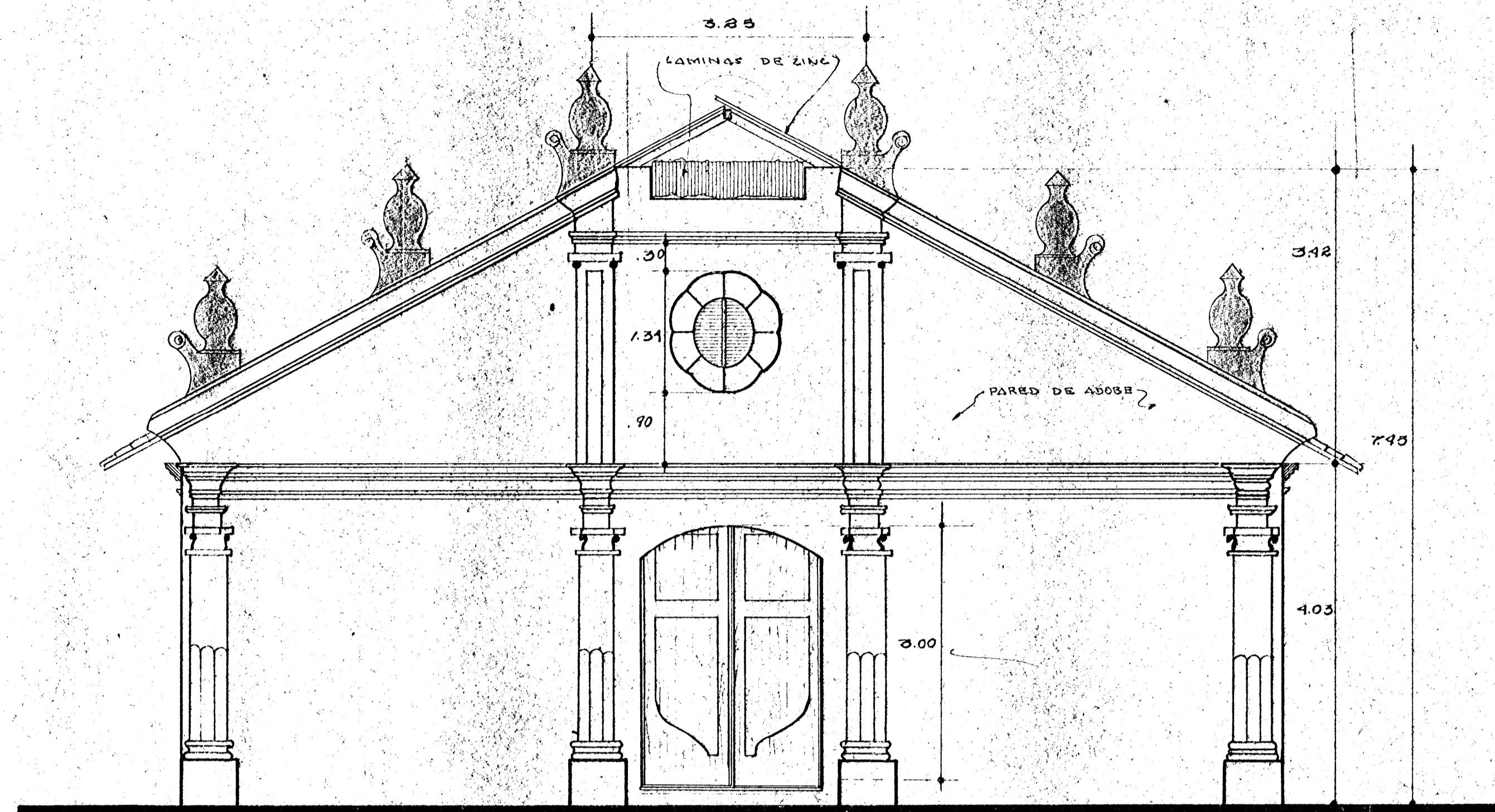
FACHADA PRINCIPAL escala 1:50
