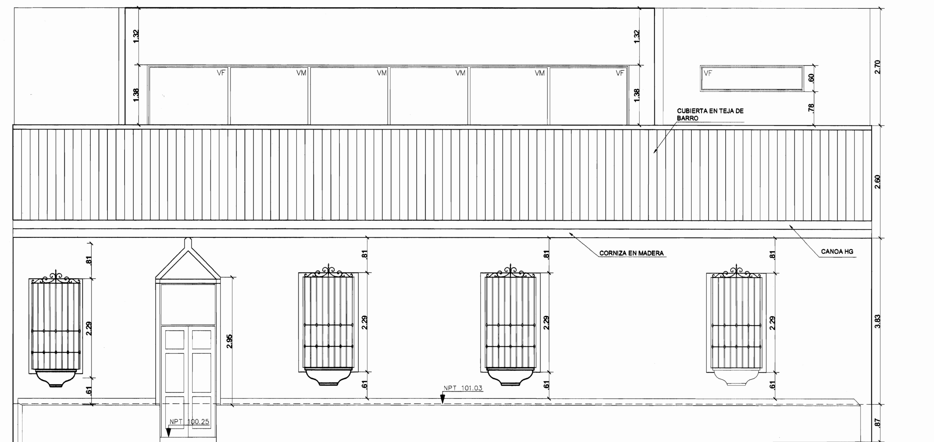
FACHADA PRINCIPAL ESCALA 1/50
